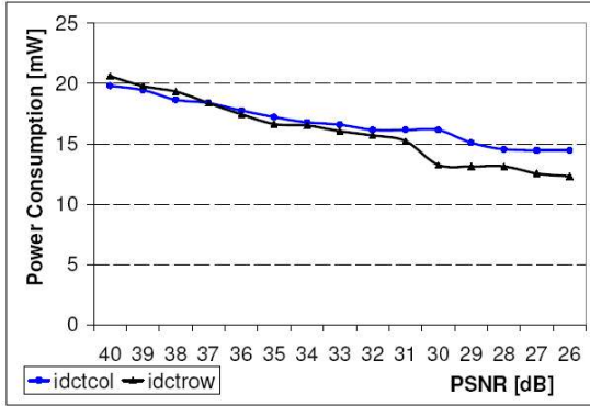
Fig. 9. Experimental Results: Power consumption with quality specification
