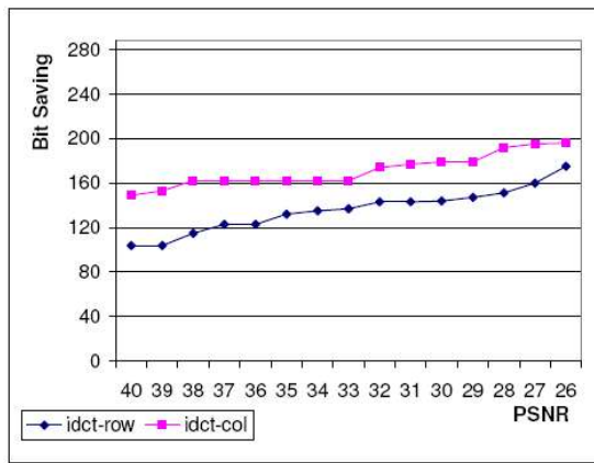
Fig. 13. Total Bitwidth Saving
