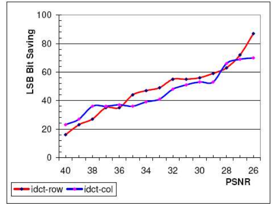
Fig. 12. Dynamic Bitwidth Saving
